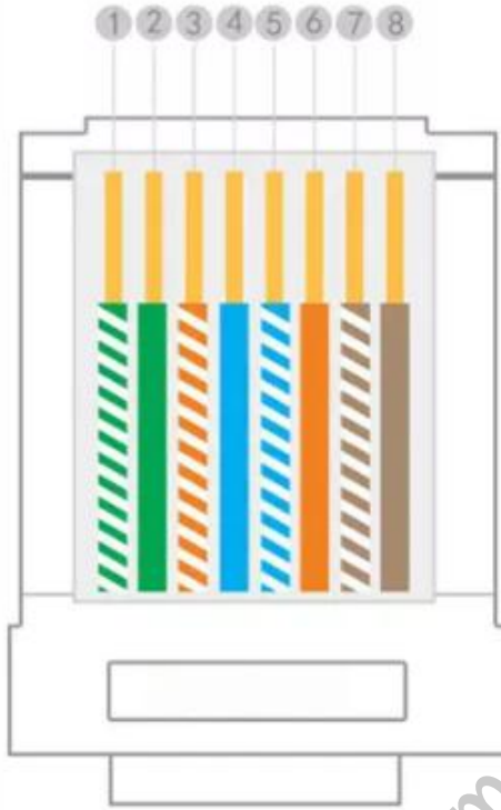
T568A Standard
