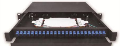
24 Core SC
